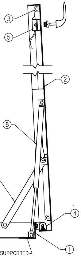
ABOVE SHOWN WITH OPTIONAL POST & CHAINS AND PADLOCK HASP
